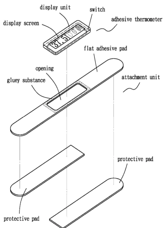
Figure 7 Decomposed view of Visual Adhesive Thermometer
