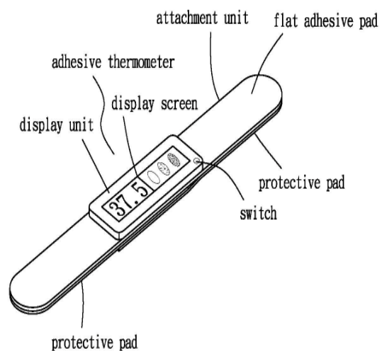
Figure 6 Exploded view of Visual Adhesive Thermometer
